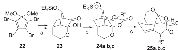
Scheme 5. Synthesis of aldehydes 25a–c . For 24 and 25 , R' = H, Me, CH 2 CH 2 OSiPh 2 tBu, for a , b , and c , respectively. Reagents and conditions: a) See the Supporting Information. b) (EtO) 2 P(O)CH(R'')COCl, Et 3 N, then NaH, THF, approximately 60 °C, 57% ( 24a ), 76% ( 24b ), 87% ( 24c ). c) Bu 4 NF, AcOH, –10 to 0 °C, 95% ( 25a ), 96% ( 25b ), 75% ( 25c ).
